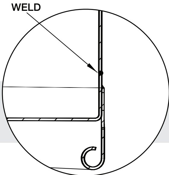
Sanitary Seamless Drum
