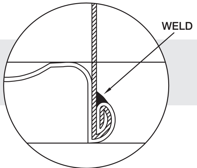
Welded or Welded Chime Drum
